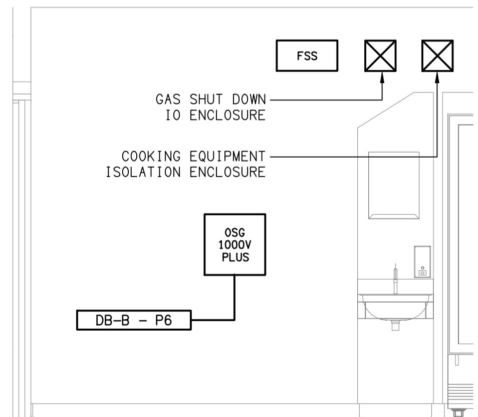
DETAIL A FIRE EQUIPMENT WALL ELEVATION SCALE: 1:25
